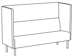
SA610/SA620/SA630 H 1230 SH 450 B 640/1390/1790 D 630
