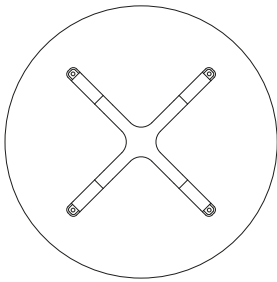
H 730/870 Ø 1800
