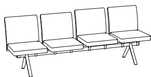
balk 4a 2 x 1-sits (sh 450) + 2 x 1-sits (sh 480) H 830/860 SH 450/480 B 2365 D 640
