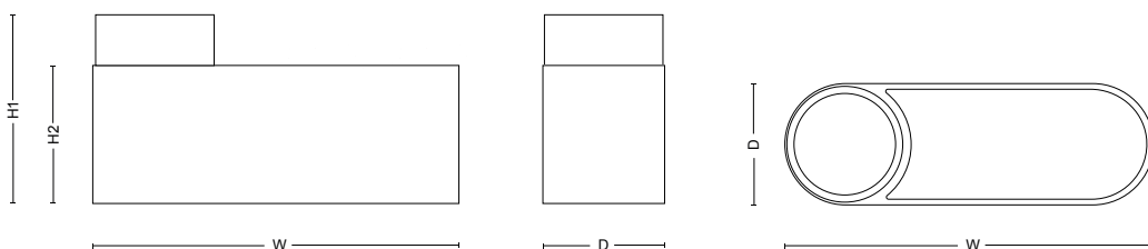
Plant Here H1 453 mm, H2 330 mm, W 874 mm, D 288 mm Art.nr. 37844xx
