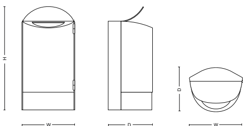
Captin H: 1023 mm, 40.3" W: 525 mm, 20.7" D: 442 mm, 17.4"
